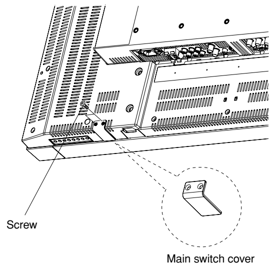
Main switch cover installation example (LDT371V)
